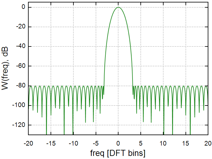
Dolph-Chebyshev window (Rs = 80 dB)
