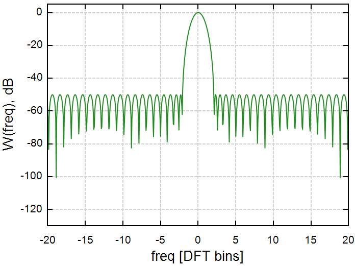
Dolph-Chebyshev window (Rs = 50 dB)
